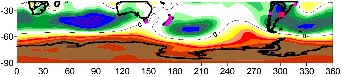
ERA-40 MSLP / Marshall (2003) SAM Correlation, 1979-2001
