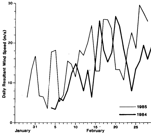
FIG. 3. Onset of winter wind conditions at Inexpressible Island.
