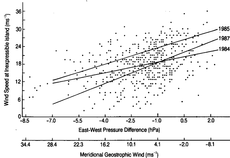
FIG. 4. Synoptic modulation of the katabatic airflow. Data for each year span the interval 15 February to 19 April. Dots represent individual three-hourly observations for 1984. Straight lines are a linear least squares fit to the data for each year.
