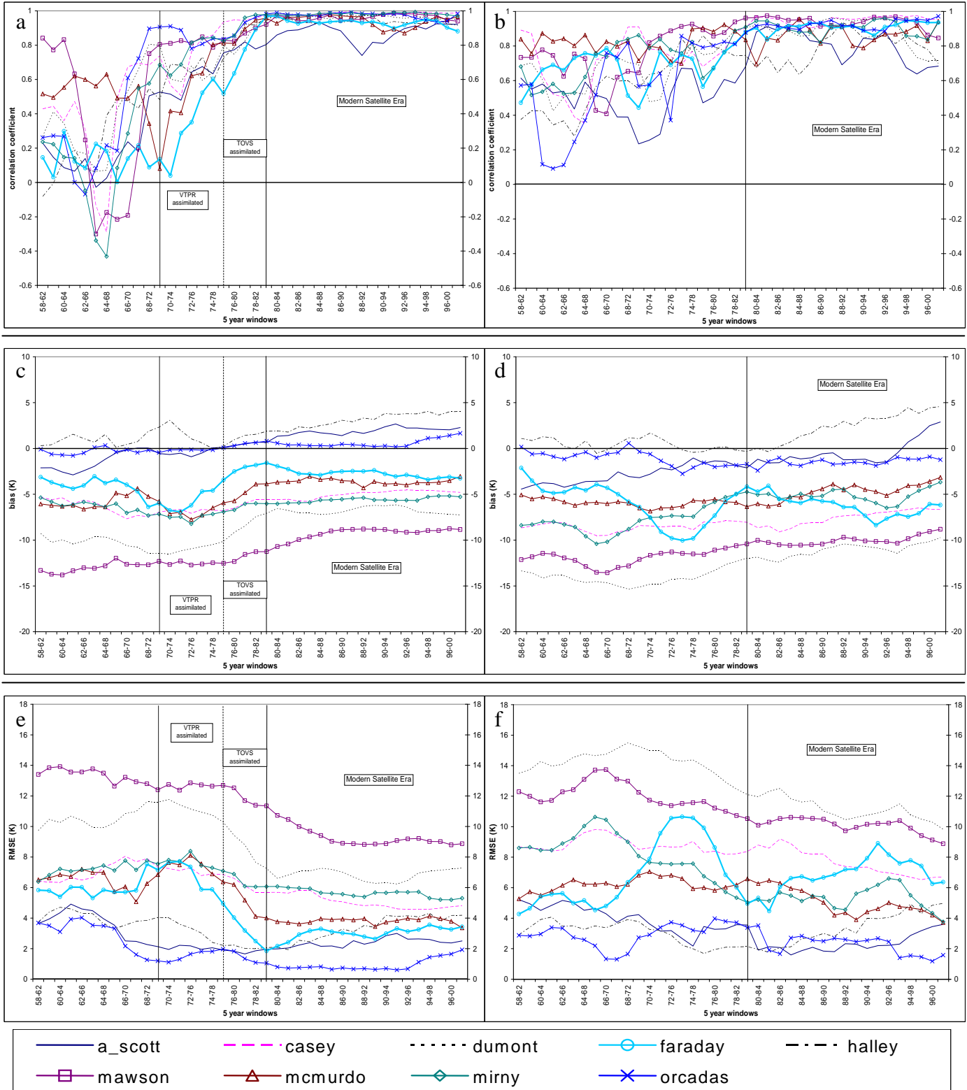
Revised Fig. 5. Same as in Fig. 3 of Bromwich and Fogt (2004), but for 2-m temperature and stations 1-9, including Faraday.
